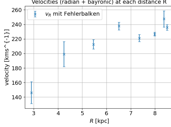
Figure 9: The radial velocity at each distance R.
