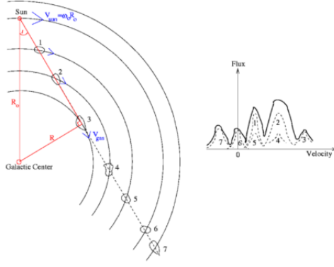
Figure 1: A schematic representation of the rotation of H1 clouds around the galactic centre together with the resulting line profile to the right [1].
